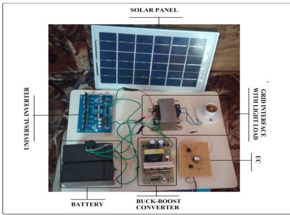
Fig. 12. Hardware setup
