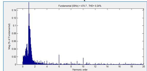
Fig.11(c). THD values of AWPI controller with Ultra-capacitor
