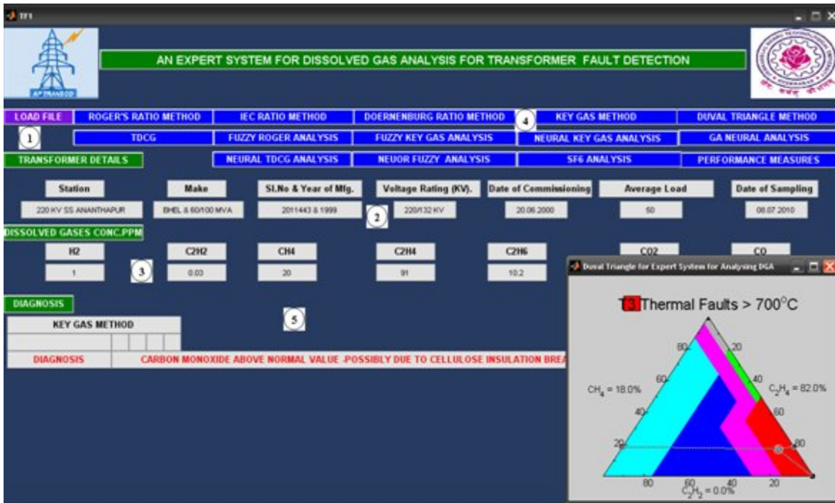
Figure (5): Snap Shot of Graphical User Interface
