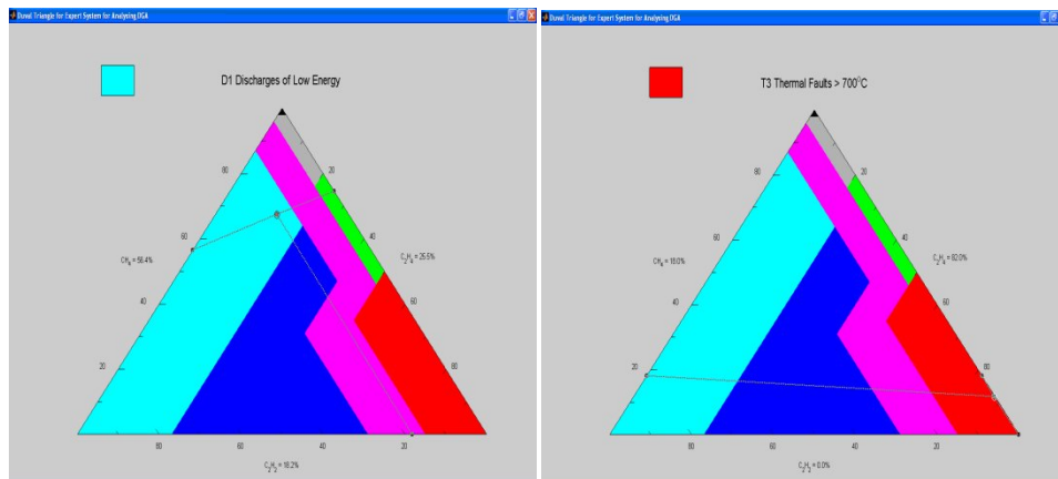
Figure (6) Snapshots of Duval Triangle for Case 1 & 2 Diagnosis as Plotted by the Tool
