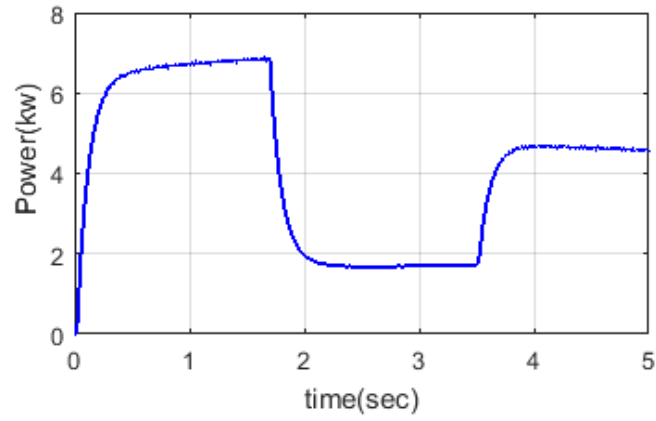
Figure.7 The measured PV input (a) irradiance and the output (b) voltage (c) current and (d) power from non-linear irradiance
